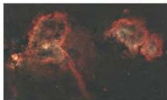
Photo of Heart and Soul Nebula, 7 Courtesy: Ed Jacoby, SCOV resident.
