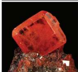
Photo Credit: Red Wulfenite from Red Cloud Mine, La Paz, AZ https://www.mindat.org/photo-270818.html
